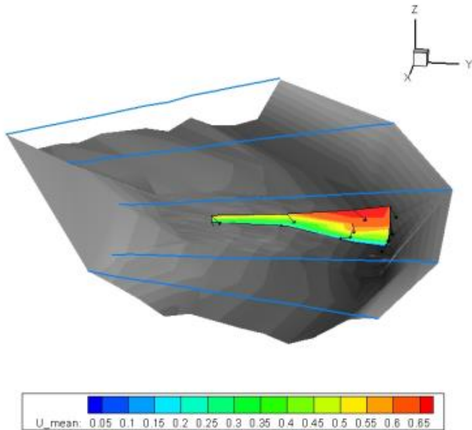
Figure 6. Velocity patterns in the mussel test section of the OSL ( U_{\text{mean}} , m/s). Flow is from top to bottom and blue lines indicate water surface. Highest velocities (up to 65 cm/s) and highest shear stresses were at the outside of the meander.
