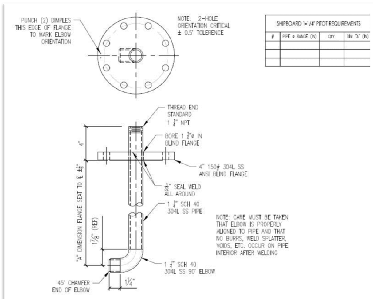
Figure 2. Diagram of Elbow Pitot for Ballast Discharge Sampling.
