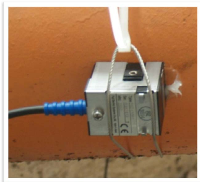
Figure 9. Flow Meter Transducer.
