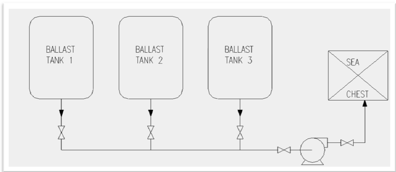
Figure 3. Schematic of Distributed Manifold Ballast System Design.
