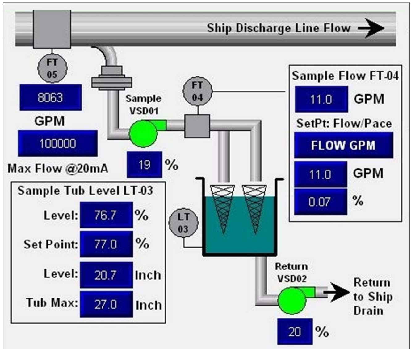
Figure 15. Sample Screen Image from GSI HMI Software.
