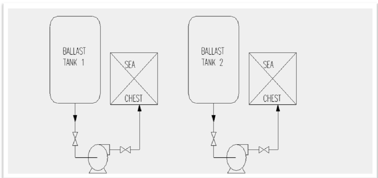
Figure 5. Schematic of Multiple Independent Ballast System Design.
