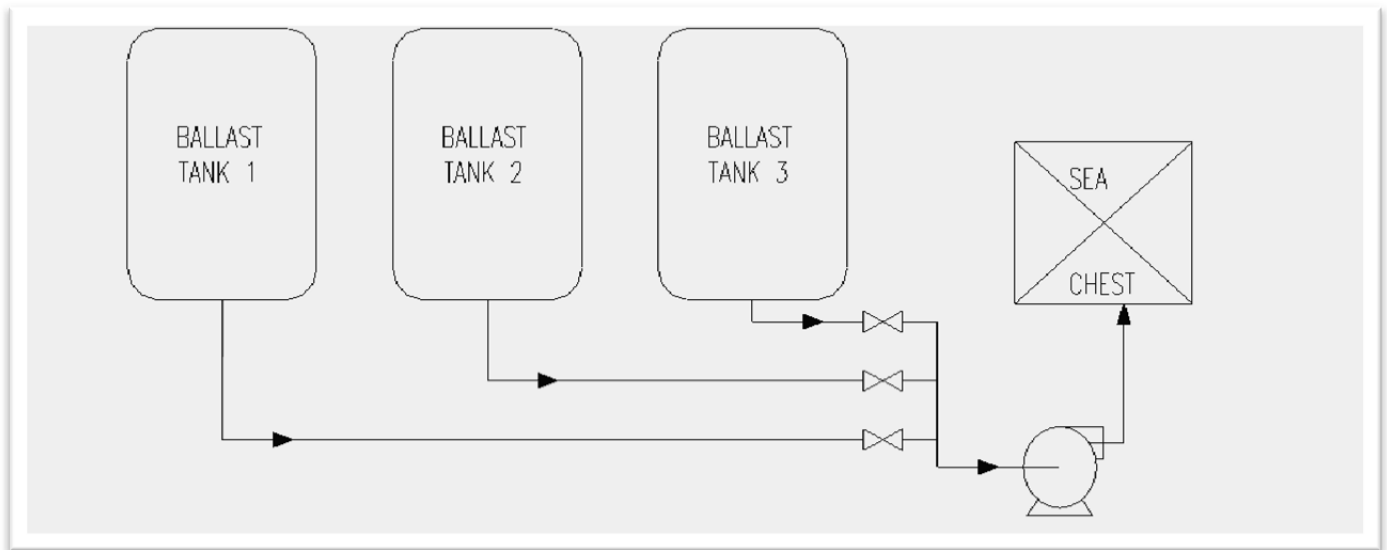
Figure 4. Schematic of Centralized Manifold Ballast System Design.
