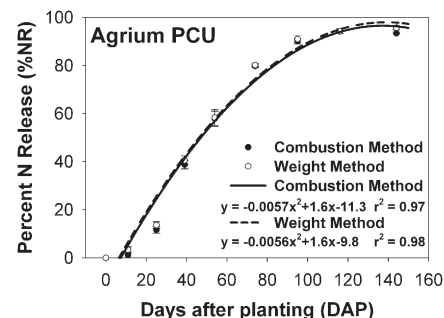
Fig. 3. Percent of nitrogen release (%NR) as a quadratic function of days after planting (DAP) for Agrium polymer-coated urea (PCU) incubated at the fertilizer band depth of the potato hill. Each point represents the mean and 1 se.
