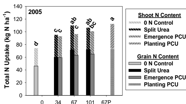
Figure 6. Total nitrogen (N) uptake in 2005 in above ground plant biomass (shoots + grain). Stacked bars with the same letters are not significantly different (p>0.10) and refer only to total N uptake.
