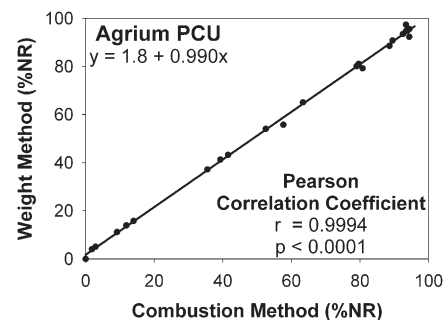
Fig. 1. The correlation between two different methods for determining percent N release (%NR) for Agrium polymer-coated urea (PCU) incubated at the fertilizer band depth of the potato hill. Each point represents one paired observation.
