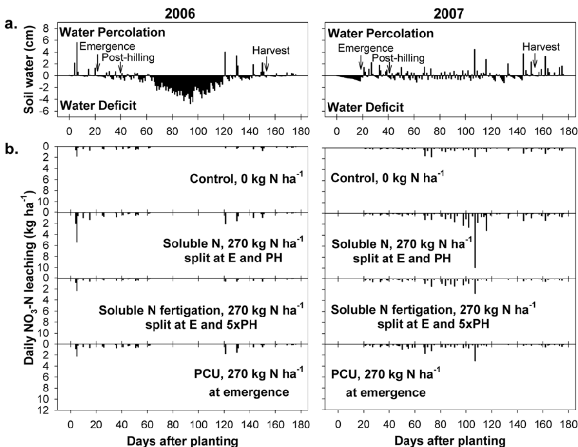
Fig. 2. Soil water balance for the top 120 cm and N source ( 270 \text{ kg N ha}^{-1} ) effect on daily nitrate leaching in 2006 and 2007. Patterns were similar for each N source at other rates and timing. Soluble N was urea at emergence and urea plus ammonium nitrate for post-hilling applications. E, emergence; PH, post-hilling; PCU, polymer-coated urea.
