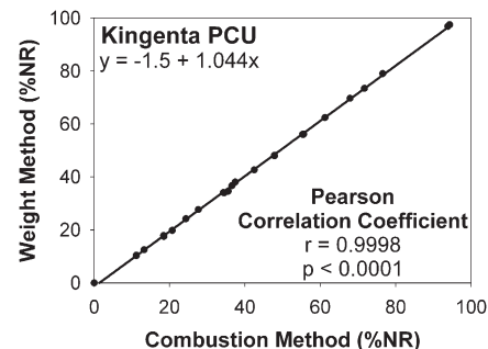
Fig. 2. The correlation between two different methods for determining percent N release (%NR) for Kingenta polymer-coated urea (PCU) incubated at the fertilizer band depth of the potato hill. Each point represents one paired observation.
