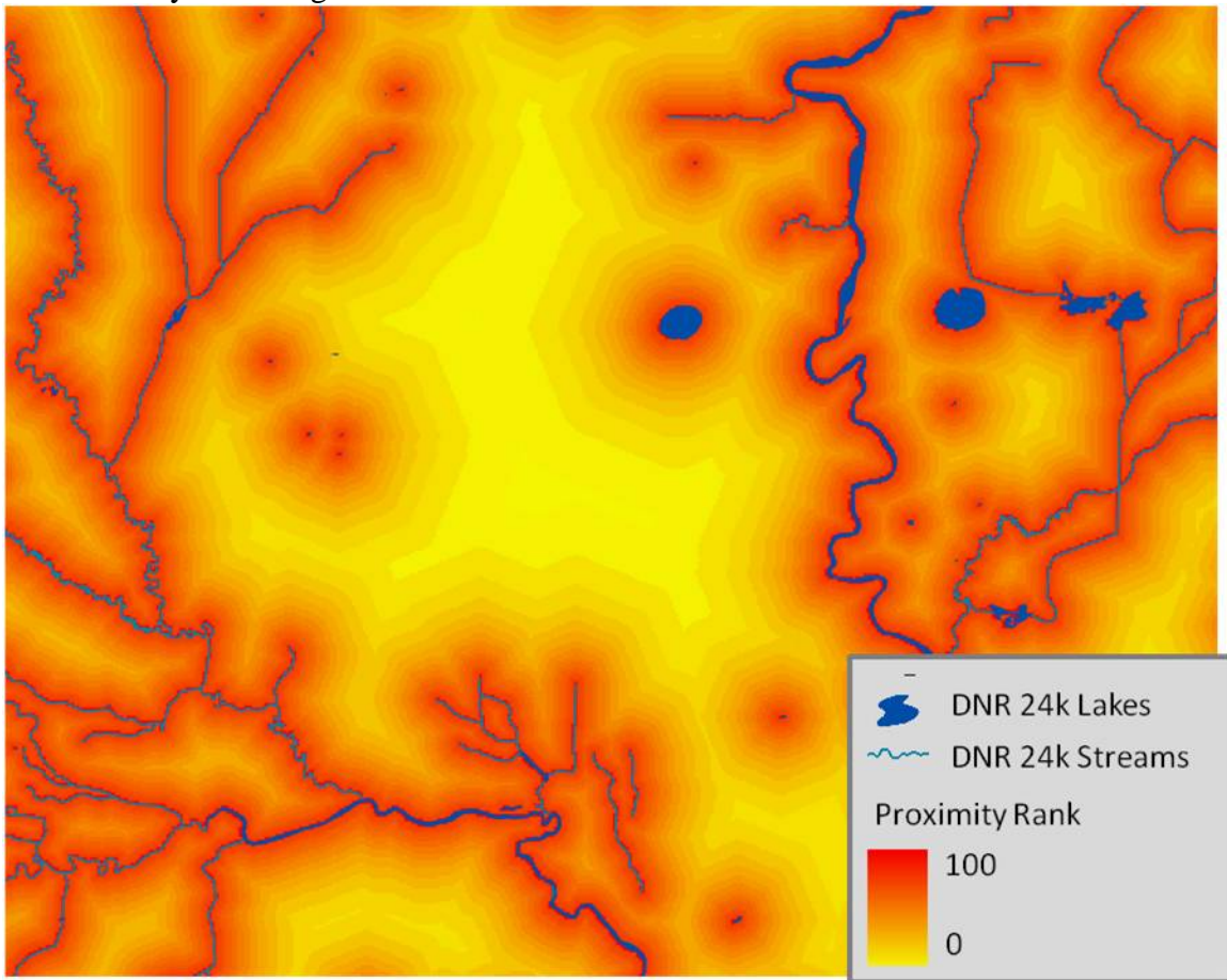
Fig. 6: Proximity of 30 m grid cells to surface water.
